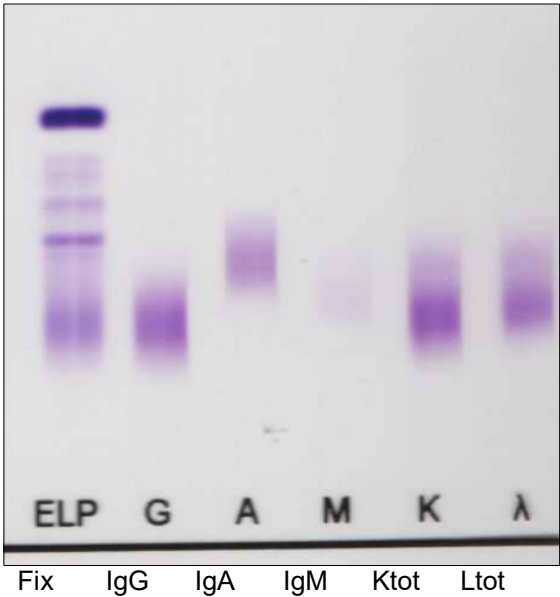
Immunofixation
